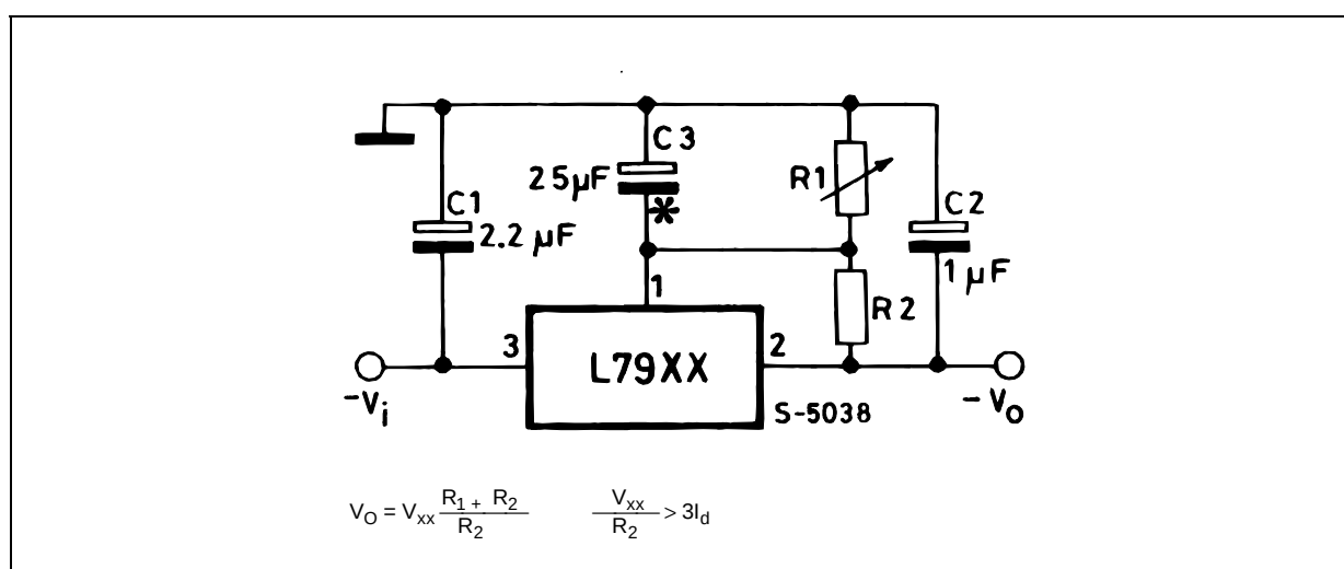
Figure 3 : Circuit for Increasing Output Voltage
