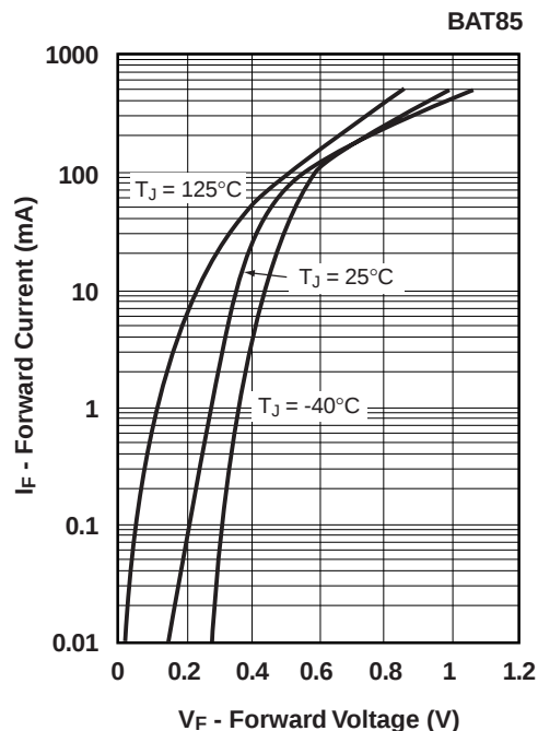
Typical Instantaneous Forward Characteristics
