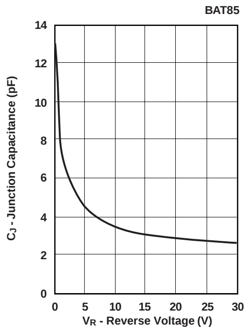
Typical Junction Capacitance
