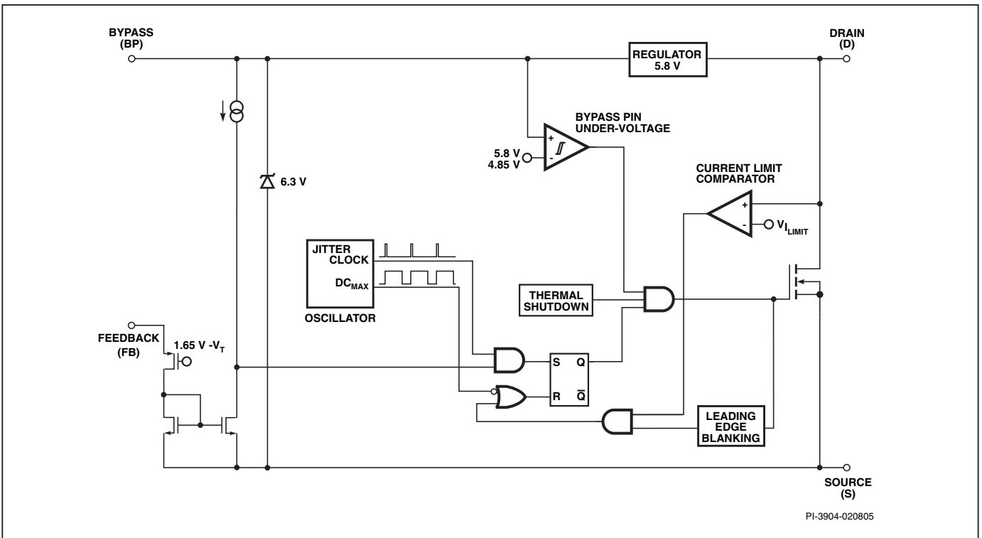
Figure 2a. Functional Block Diagram (LTK302).
