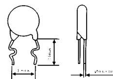
Type(c)-kink Type
