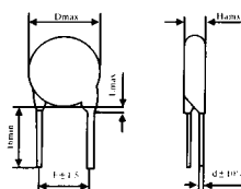
Type(b)-straight Lead
