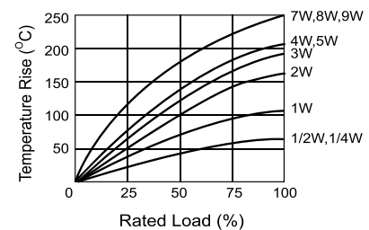
Heat Rise Chart
