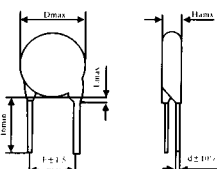
Type(b)-straight Lead
