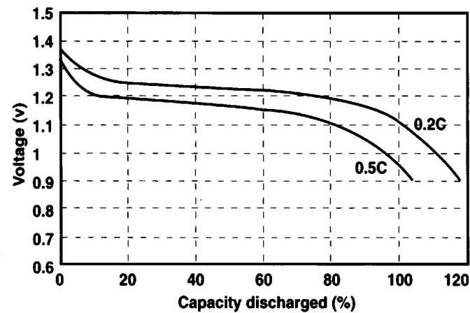
Discharge curves of single cell EH-60B16 at -80mAh at various discharge rates at room temperature.
