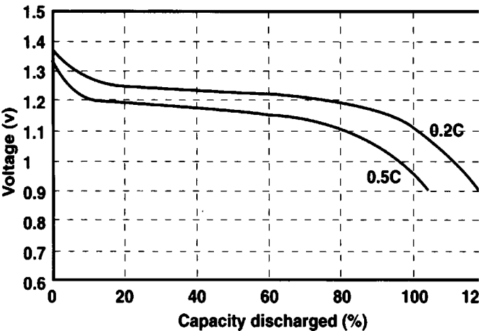
Discharge curves of single cell EH-60B16 at -8( at various discharge rates at room temperatu
