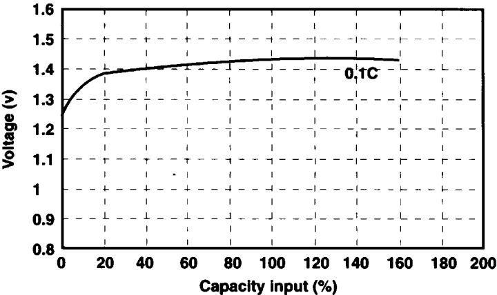
Charging curve of single cell EH-60B16-80mAh at 0.1C charging rate
