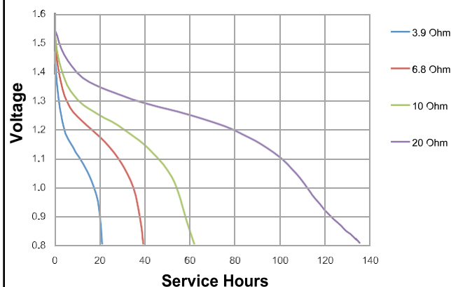
Constant Resistance
