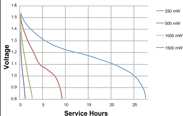
Constant Power
