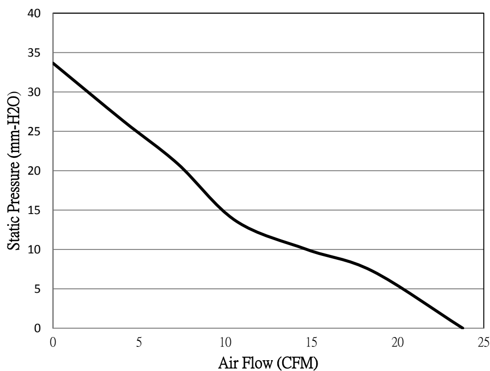
P-Q Curve
