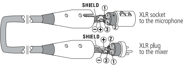
BALANCED AND SHIELDED MICROPHONE CABLE WITH XLR CONNECTORS:
