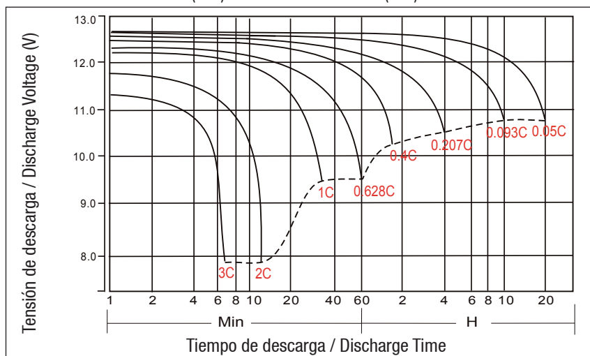
CURVAS DE DESCARGA A 25°C (77°F) DISCHARGE CURVES 25°C (77°F)
