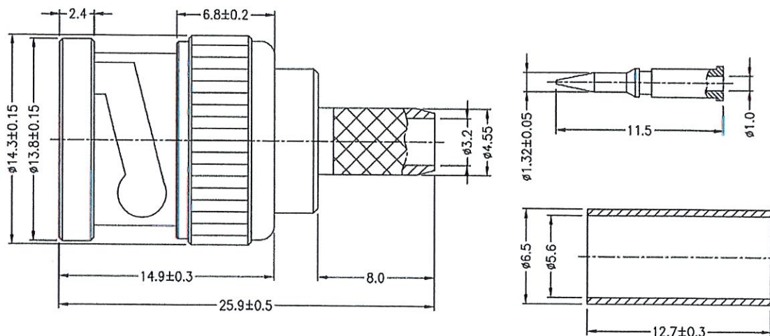
Catalogue Drawing:
