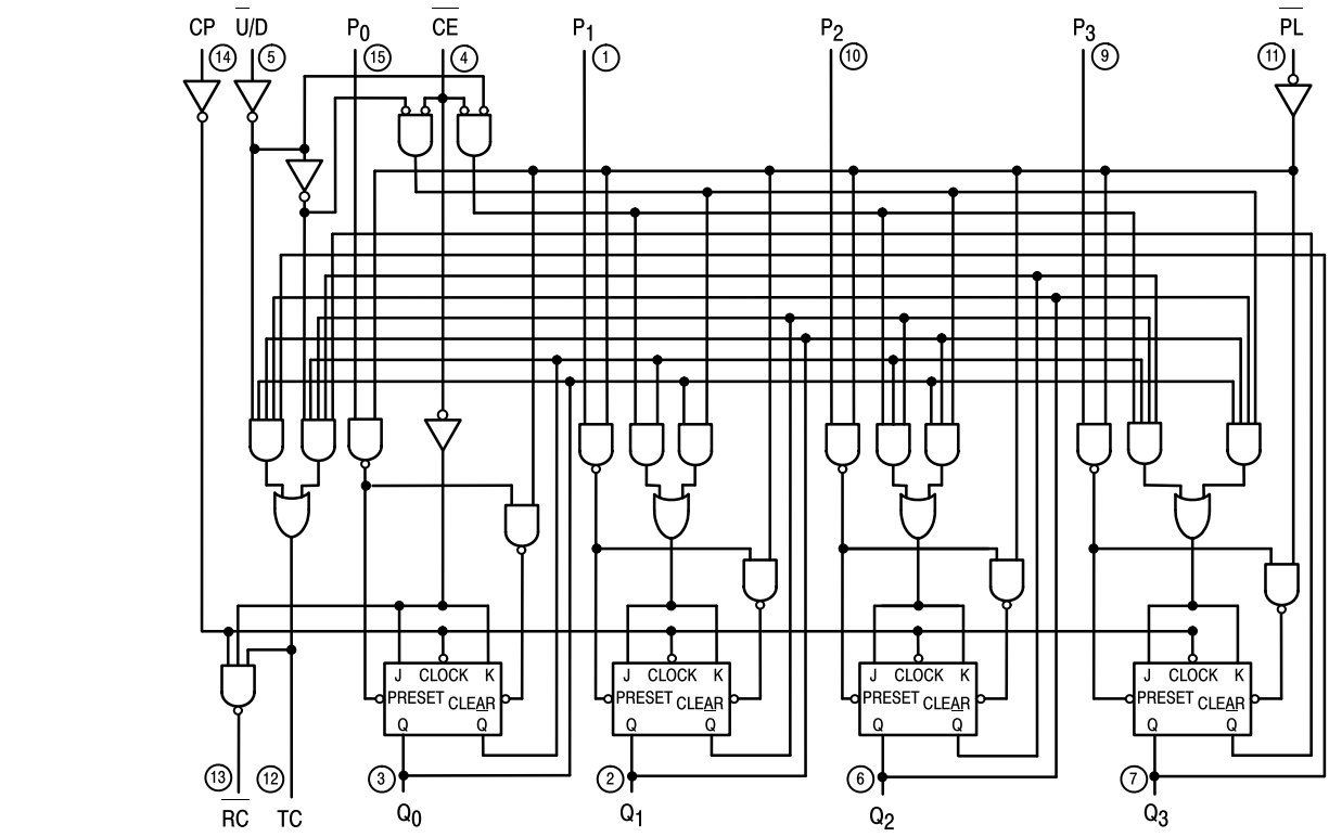
BINARY COUNTER LS191
