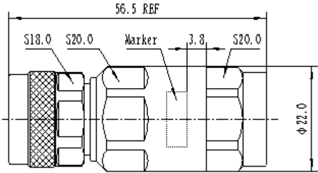
NM-LCF12-C03 Outline Drawing
