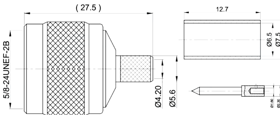
Catalogue Drawing:
